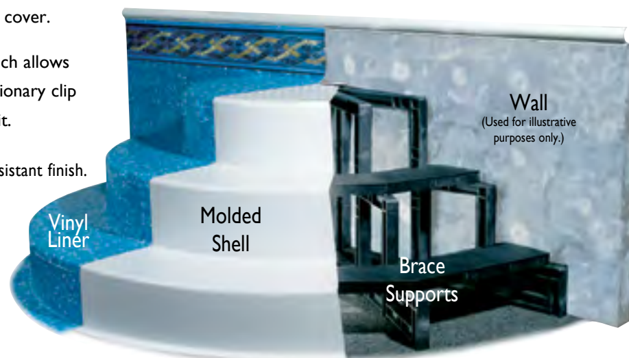
180° Straight Step Cutaway
